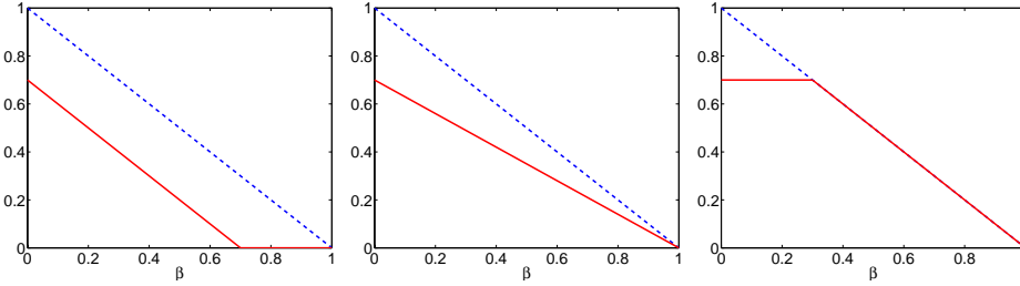
Figure 3: Modification of \mathcal{S}_-(x) = 1 - \beta (dashed line) by shifting (Lukasiewicz, left), scaling (Reichenbach, middle), or bounding (Kleene-Dienes, right) in the case \alpha = 0.7 .
